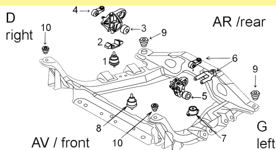
9001385 Support moteur D OE 1J0199262BE Right engine mounting
